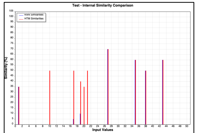
Fig. 11: Internal Similarity plot for test data (case 2)
