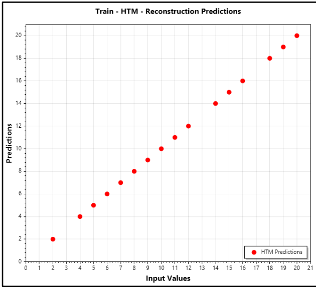
Fig. 13: HTM reconstruction plot for train data (case 1)
