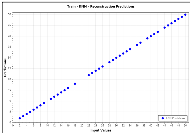
Fig. 16: KNN reconstruction plot for train data (case 2)
