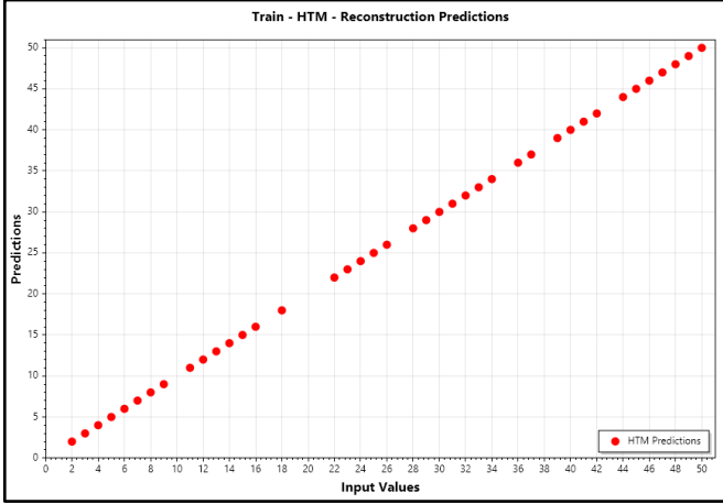
Fig. 17: HTM reconstruction plot for train data (case 2)
