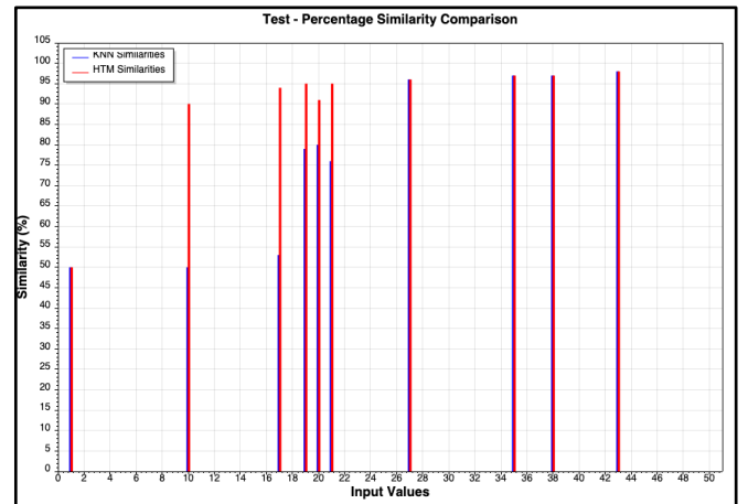
Fig. 10: Percentage Similarity plot for test data (case 2)
