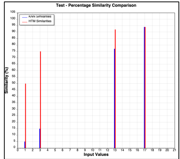
Fig. 6: Percentage Similarity plot for test data (case 1)
