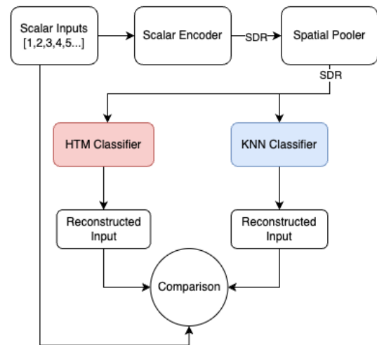
Fig. 1: Experiment Flow Diagram
