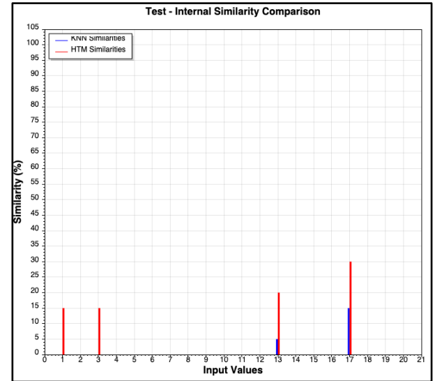
Fig. 7: Internal Similarity plot for test data (case 1)
