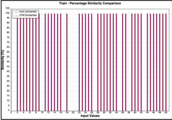
Fig. 18: Percentage Similarity plot for train data (case 2)
