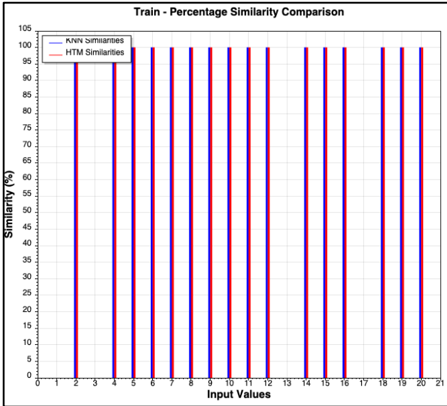
Fig. 14: Percentage Similarity plot for train data (case 1)
