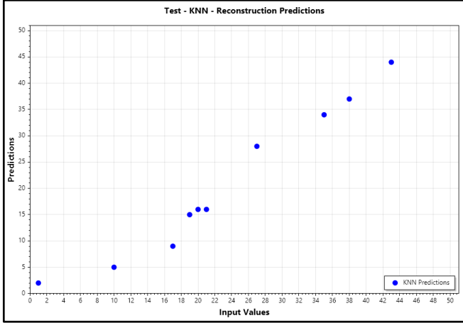
Fig. 8: KNN reconstruction plot for test data (case 2)
