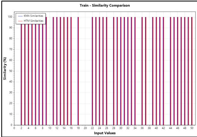
Fig. 15: Similarity plot for train data (case 2)
