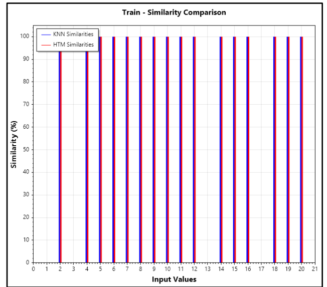
Fig. 12: Similarity plot for train data (case 1)
