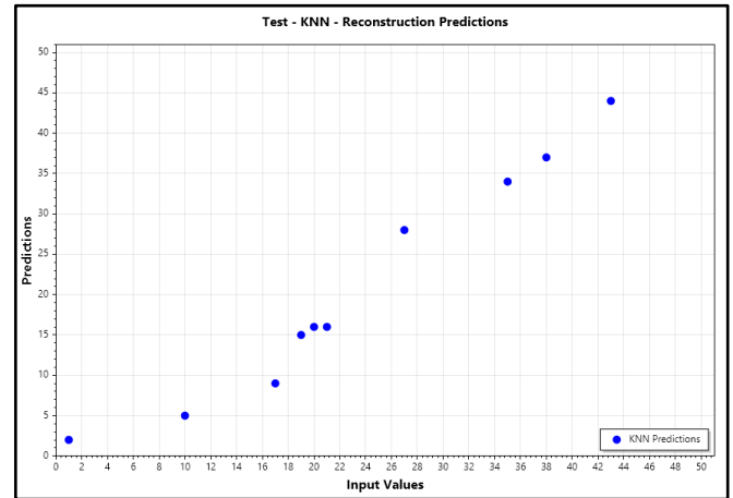
Fig. 7: KNN reconstruction plot for test data (case 2)
