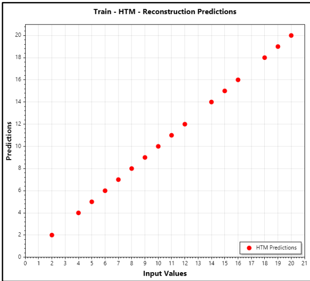
Fig. 11: HTM reconstruction plot for train data (case 1)
