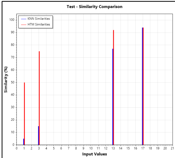
Fig. 6: Similarity plot for test data (case 1)
