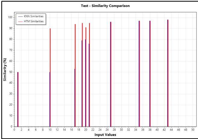
Fig. 9: Similarity plot for test data (case 2)
