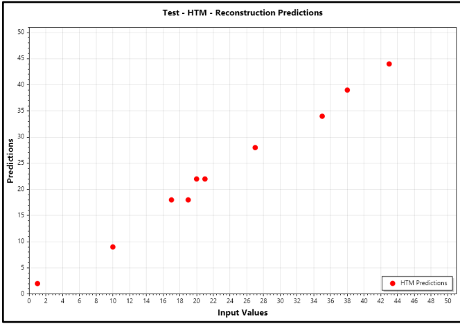
Fig. 8: HTM reconstruction plot for test data (case 2)
