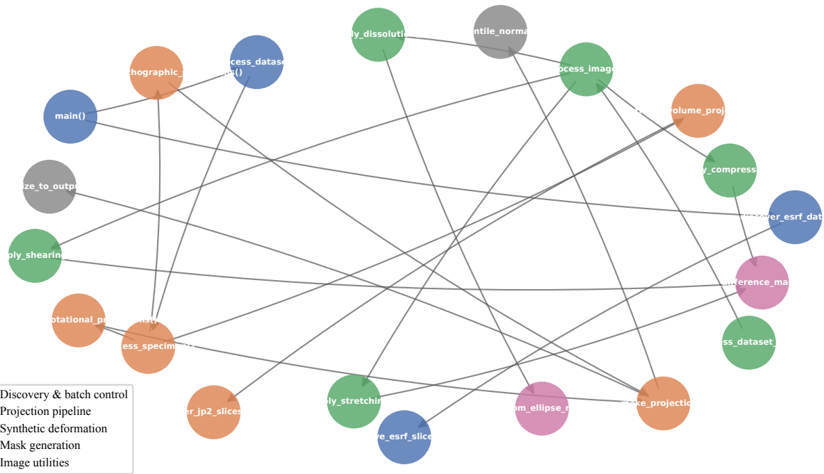
TDE Key Function Call Graph
