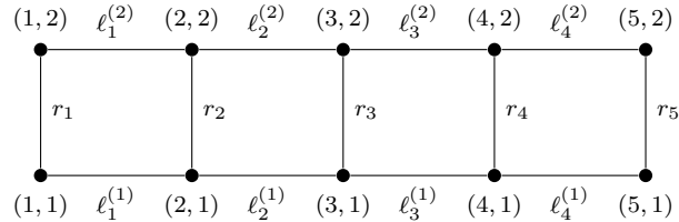
Figure 1: The ladder \mathcal{L}_5 with its edge labels.
