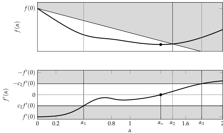
Figure 26.1: The Wolfe conditions for line search termination. Optimisation utility f(\alpha) and f'(\alpha) as black curves (top and bottom figure, respectively). True optimal step \alpha_* is marked by a black circle. The sufficient-decrease condition excludes the grey region in the top figure, constraining the acceptable space to [0, \alpha_2] . Adding the weak curvature condition additionally excludes the lower grey region in the bottom plot (thus restricting the acceptable space now to [\alpha_1, \alpha_2] ). The strong extension also excludes the top region (restricting to [\alpha_1, \min\{\alpha_2, \alpha_3\}] ). All points in between are considered acceptable by the Wolfe conditions. In this example, the true extremum lies within that acceptable region, but this is not guaranteed by the conditions. (For this plot, the parameters were set to c_1 = 0.4, c_2 = 0.5 to get an instructive plot. These are not particularly smart choices for practical problems; see the end of §26.2.)
