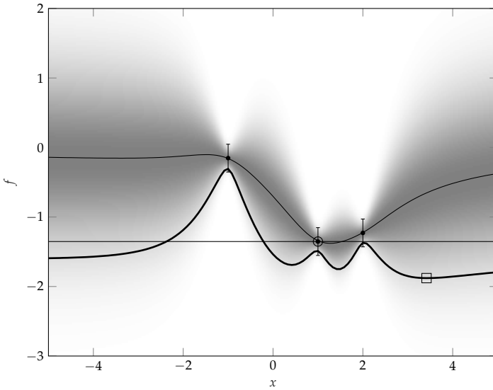
Figure 33.2: The upper confidence bound (UCB) acquisition function at x is a linear combination of the mean and standard deviation (SD) of the GP posterior. For the purposes of this plot, \beta = 1.5 . On a grid of example locations, the plot shows as a dark, thick, line the resulting acquisition function \alpha_{\text{UCB}}(x) affinely rescaled for visualisation. Its maximiser, marked with a square, gives the best possible location for the next evaluation, x_n . The plot is analogous to that for EI in Figure 32.1 and PI in Figure 33.1. Note the subtle differences between the three acquisition functions: in particular, UCB (for \beta = 1.5 ) is the most explorative of the three.
