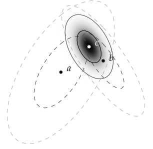
Figure 3.1: The product of two Gaussian densities is another Gaussian density, up to normalisation.
