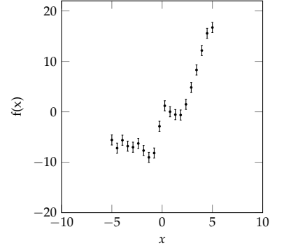
Figure 4.1: A simple nonlinear data set with i.i.d. Gaussian observation noise, i.e. \Lambda = \sigma^2 I_N , \sigma \in \mathbb{R}_+ (error-bars). Figures 4.2 and 4.3 demonstrate the effect of varying prior assumptions on the posterior induced by these observations.
