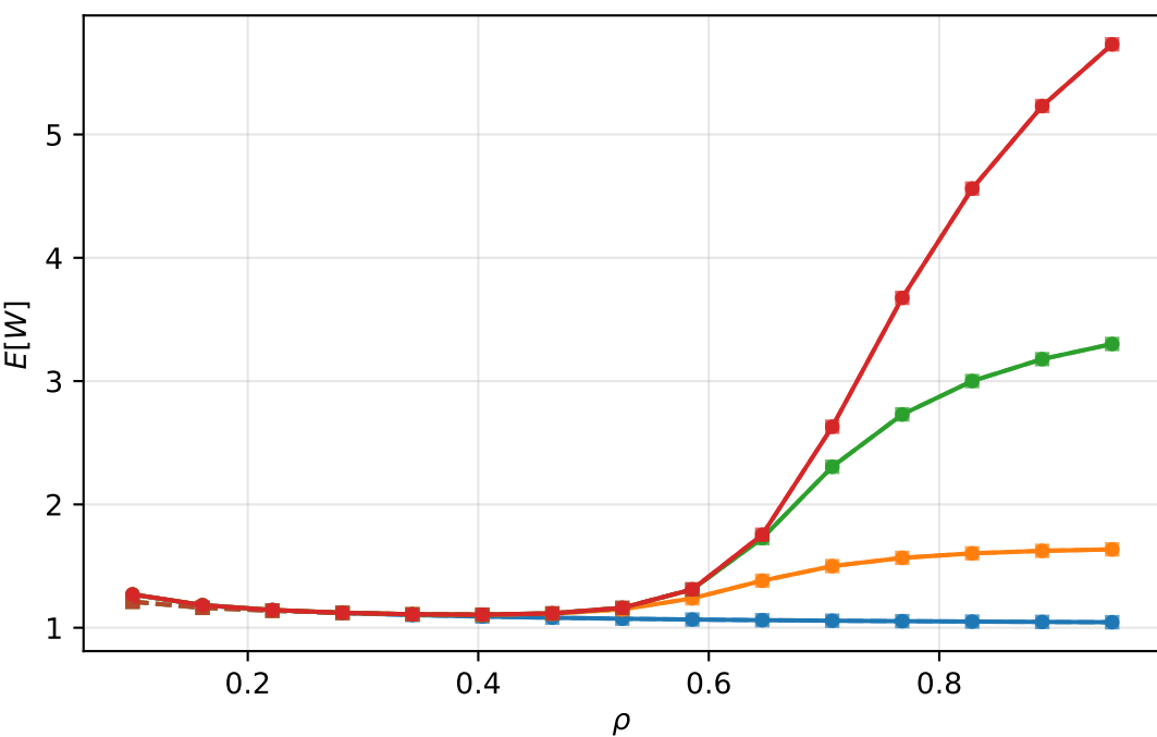
Experiment 4 vs 4-P (medium burst): Base vs Predictive (medium burst, n target=10, gamma=1.0)
