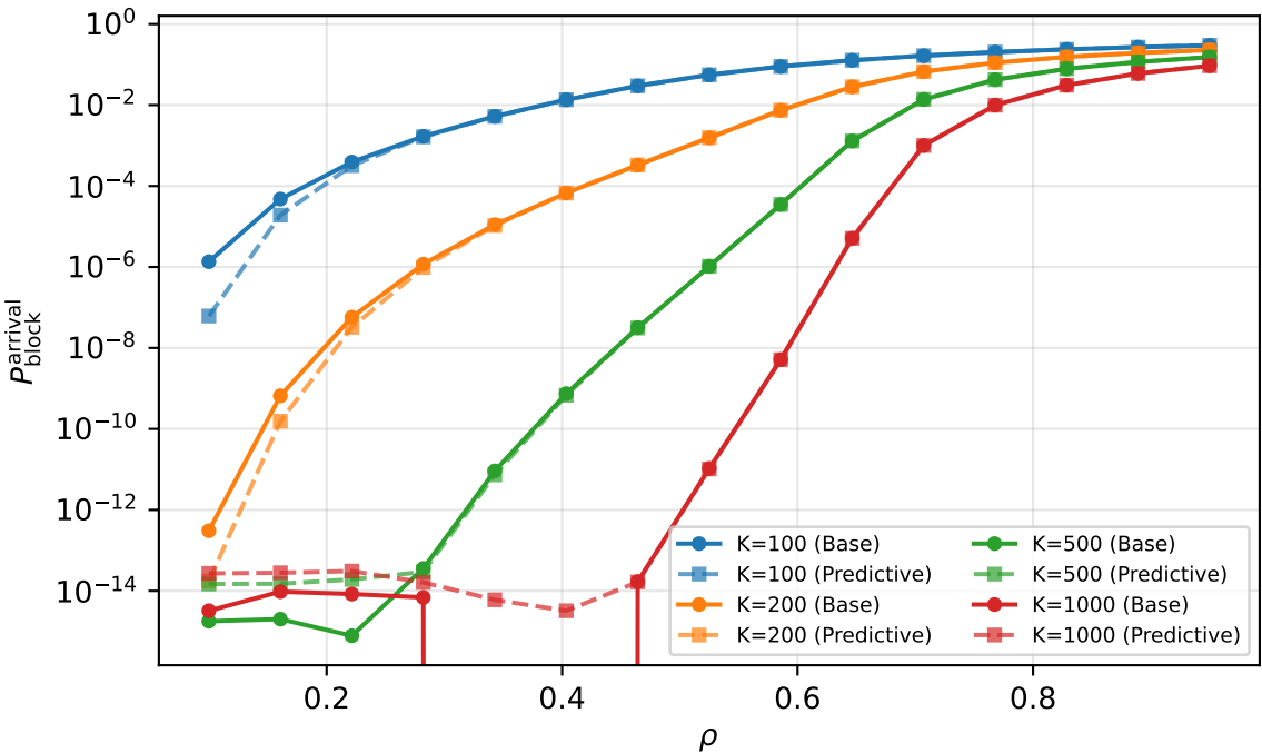
Experiment 4 vs 4-P (medium burst): Base vs Predictive (medium burst, n target=10, gamma=1.0)
