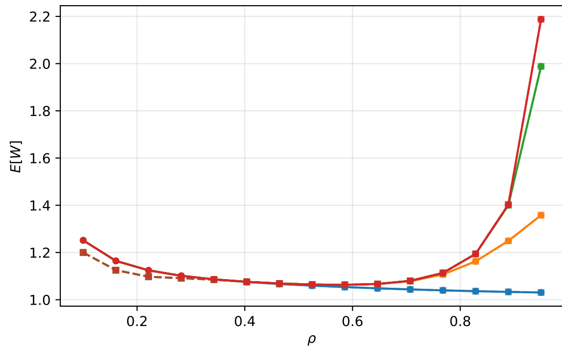
Experiment 4 vs 4-P (weak burst): Base vs Predictive (weak burst, n_target=10, gamma=1.0)
