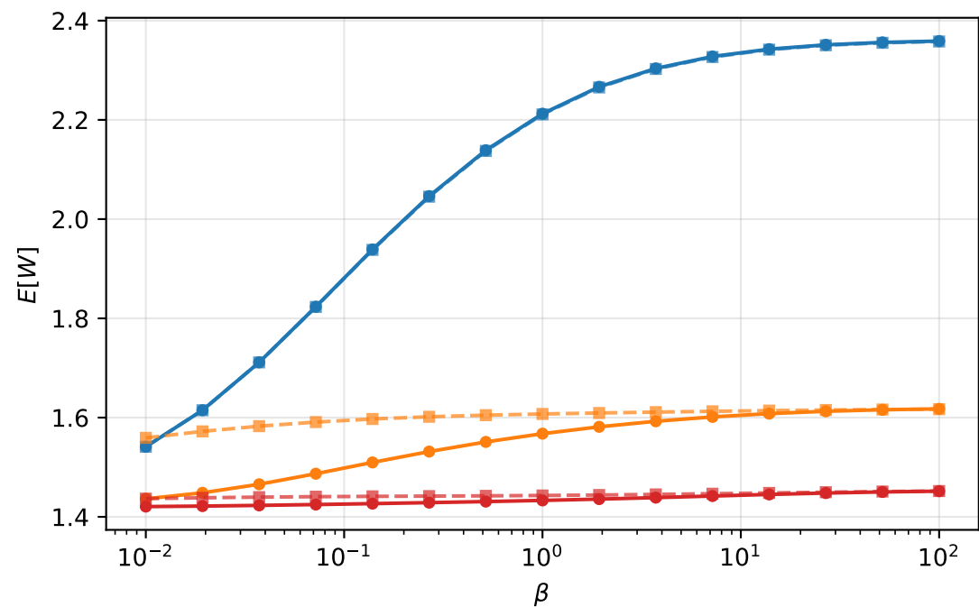
Experiment 2 vs 2-P (medium burst): Base vs Predictive (medium burst, n_{\text{target}}=10 , \gamma=\alpha\text{-map} )
