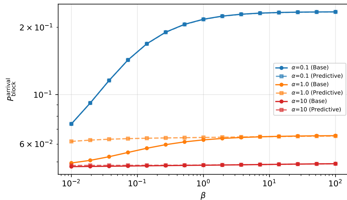
Experiment 2 vs 2-P (medium burst): Base vs Predictive (medium burst, n_{\text{target}}=10 , \gamma=\alpha\text{-map} )
