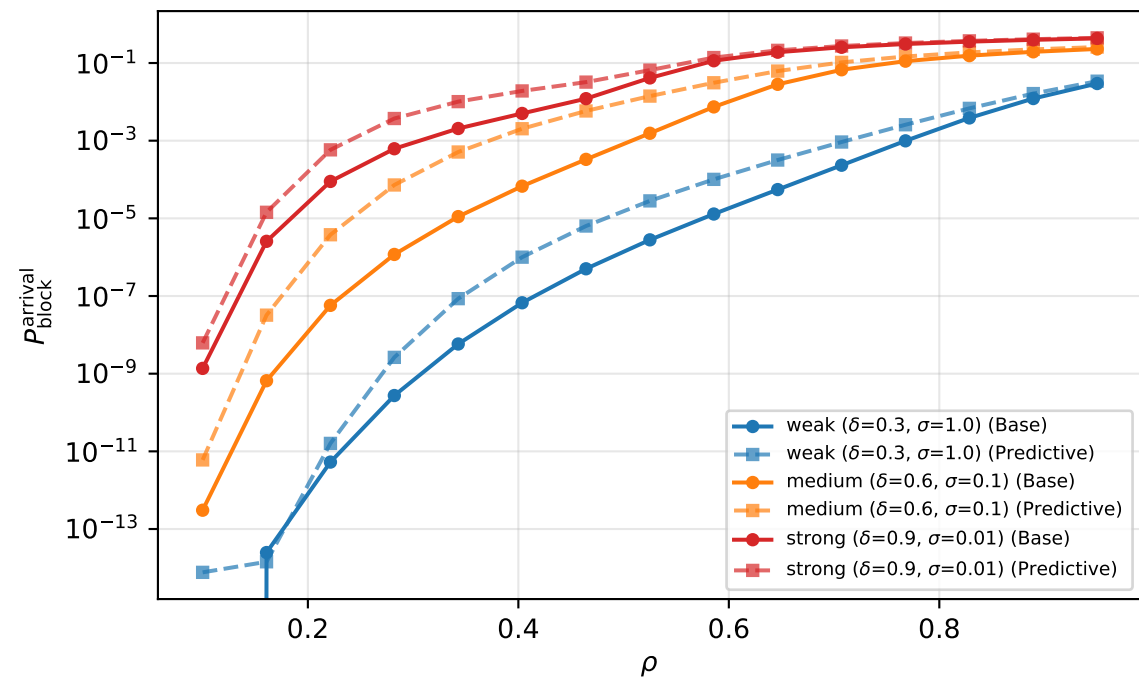
Experiment 1 vs 1-P: Base vs Predictive (n_target=10, gamma=5.0)
