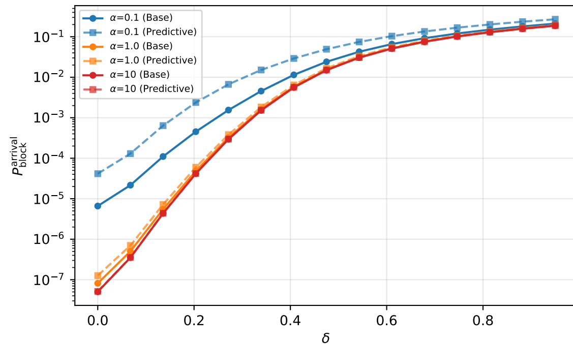
Experiment 3-A vs 3-P-A (delta sweep): Base vs Predictive (delta sweep, n_target=10, gamma=5.0)
