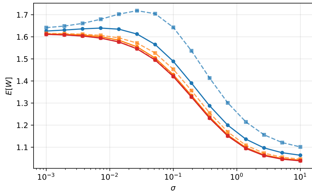
Experiment 3-B vs 3-P-B (sigma sweep): Base vs Predictive (sigma sweep, n_target=10, gamma=5.0)
