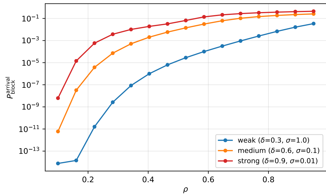
Experiment 1-P: Predictive Response to Traffic Intensity \rho ( c=20 , K=200 , b=5 , 1/\alpha=10s , 1/\beta=200s , n_{\text{target}}=10 , \gamma=5.0 )
