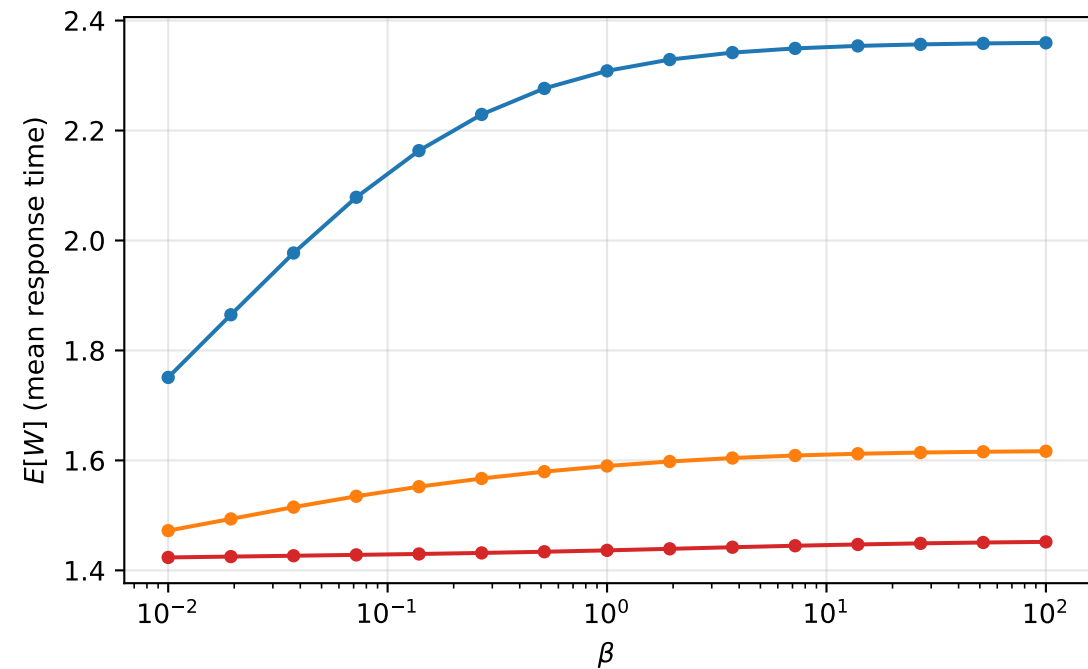
Experiment 2-P: Predictive Response to Delayoff Rate \beta (medium burst) (c=20, K=200, b=5, rho=0.7, n_target=10, gamma=5.0)
