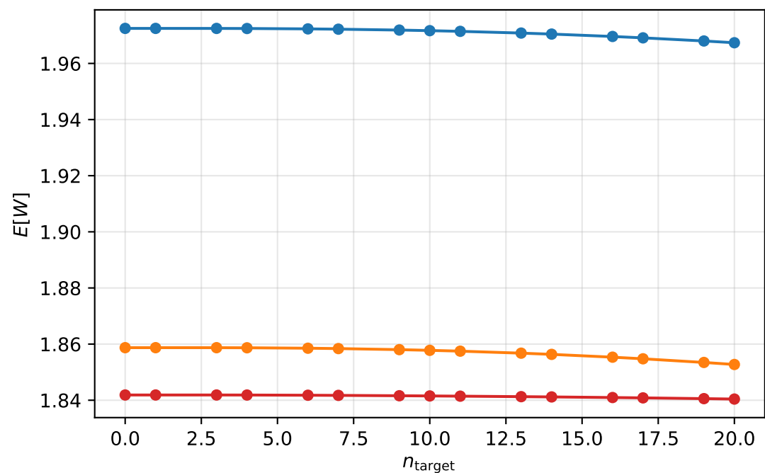
Experiment 5: Sensitivity to n_{\text{target}} (strong burst, \gamma=5.0 ) ( c=20 , K=200 , b=5 , \rho=0.7 )
