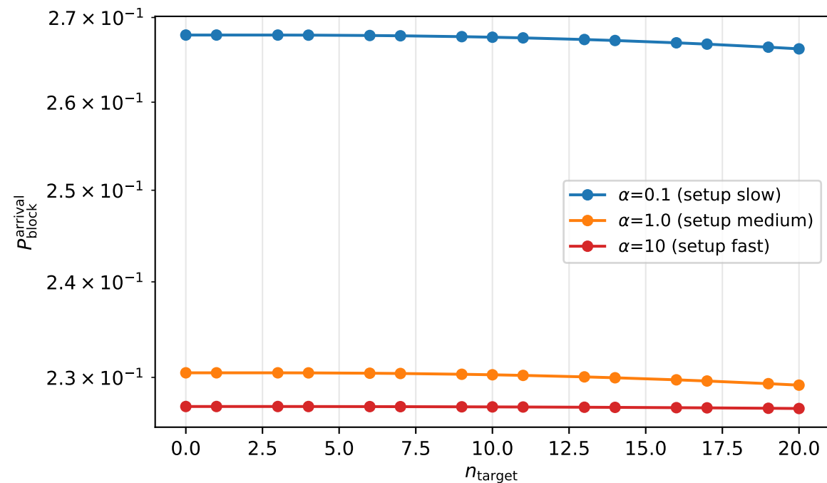
Experiment 5: Sensitivity to n_{\text{target}} (strong burst, \gamma=5.0 ) ( c=20 , K=200 , b=5 , \rho=0.7 )
