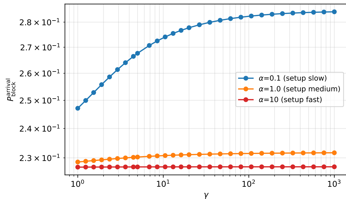
Experiment 6 (Extended): Sensitivity to gamma (strong burst, n_{\text{target}}=10 ) \gamma \in [1, 1000] , initial + extended sweeps merged
