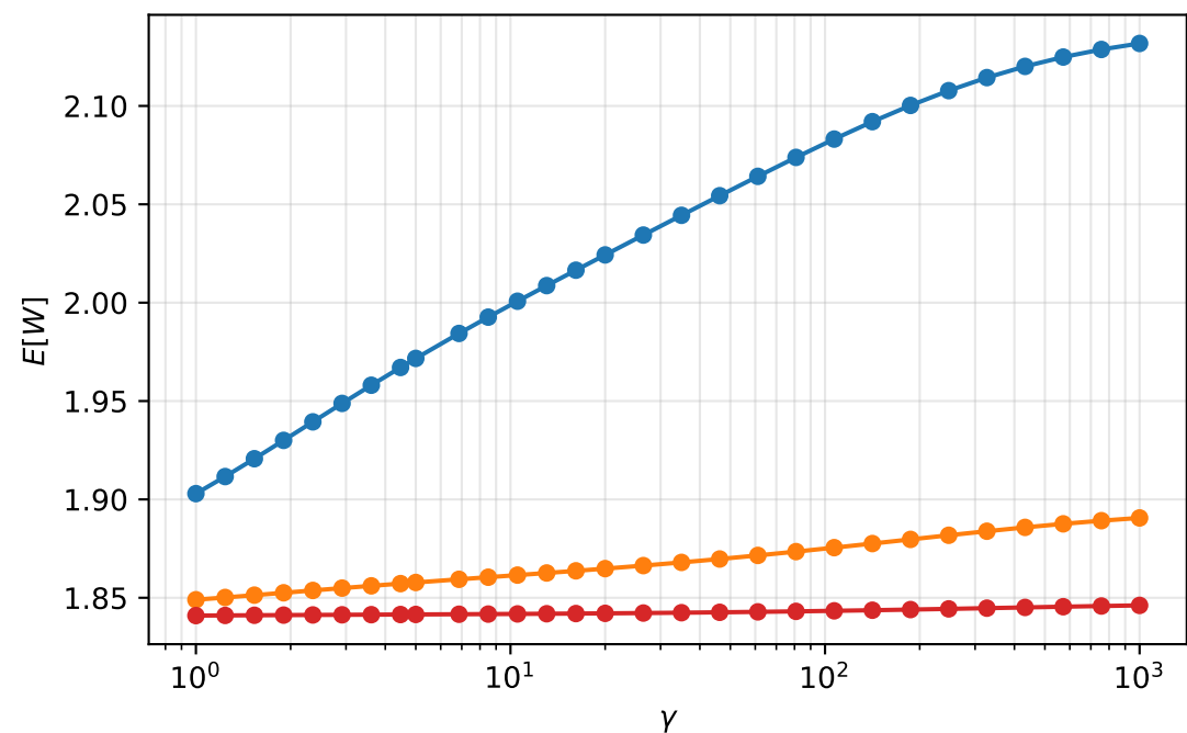
Experiment 6 (Extended): Sensitivity to gamma (strong burst, n_{\text{target}}=10 ) \gamma \in [1, 1000] , initial + extended sweeps merged
