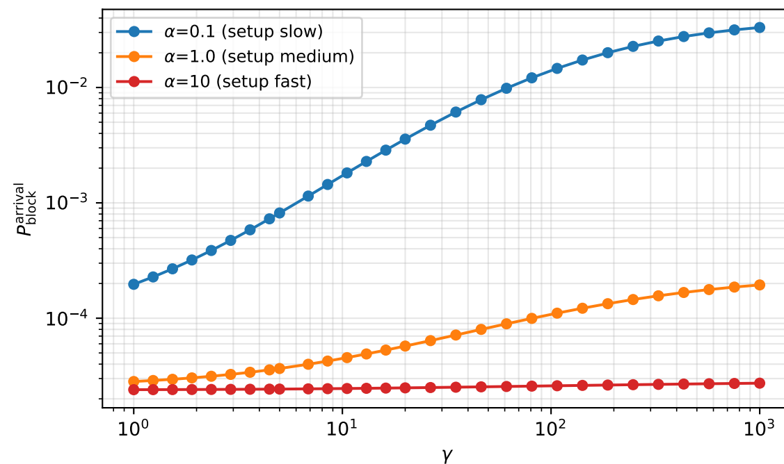
Experiment 6 (Extended): Sensitivity to gamma (weak burst, n_{\text{target}}=10 ) \gamma \in [1, 1000] , initial + extended sweeps merged
