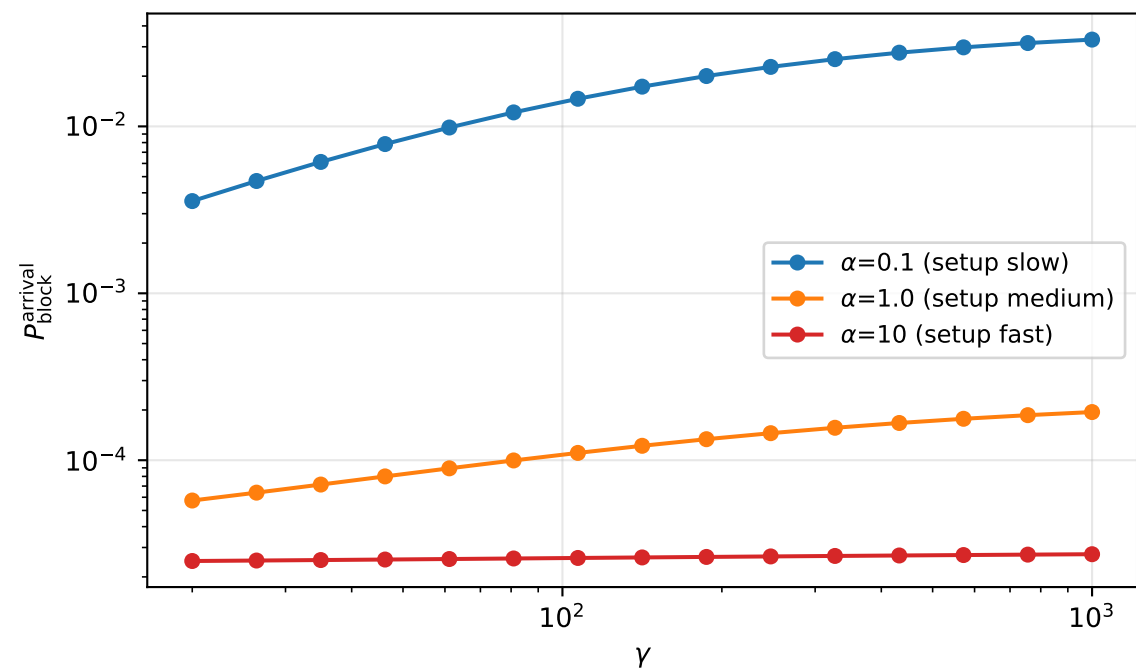
Experiment 6: Sensitivity to gamma (weak burst, n_{\text{target}}=10 ) ( c=20 , K=200 , b=5 , \rho=0.7 )
