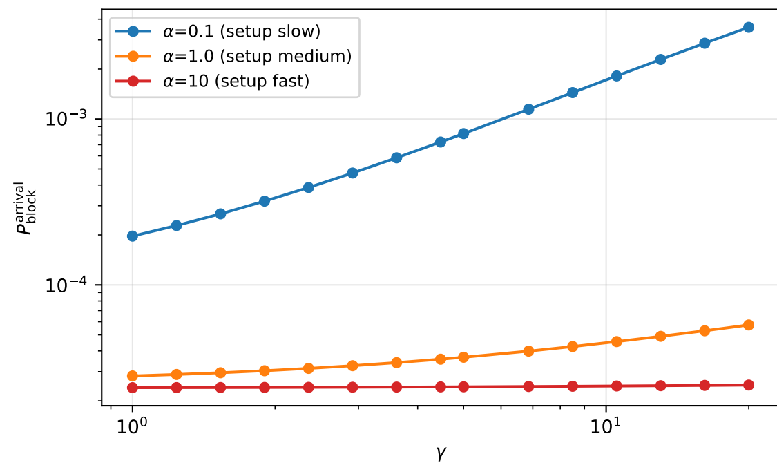
Experiment 6: Sensitivity to gamma (weak burst, n_{\text{target}}=10 ) ( c=20 , K=200 , b=5 , \rho=0.7 )
