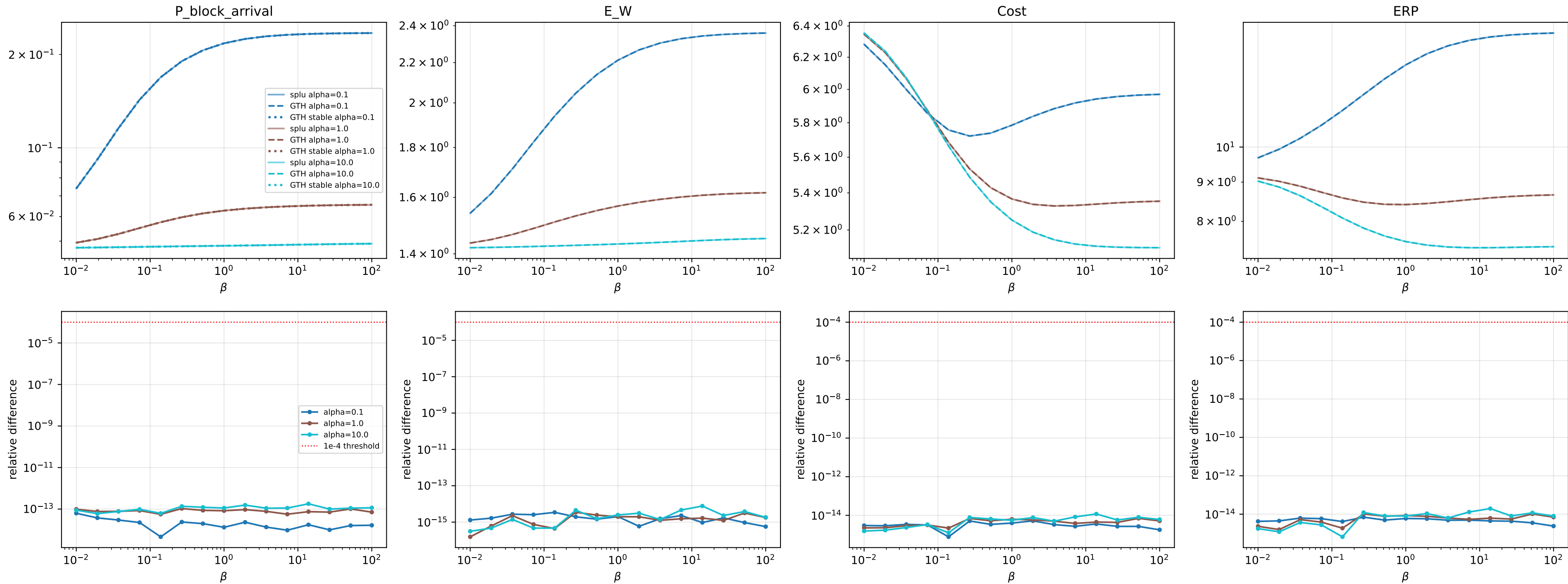
experiment_2_medium: splu (old, solid) vs GTH (new, dashed); bottom row = relative difference
