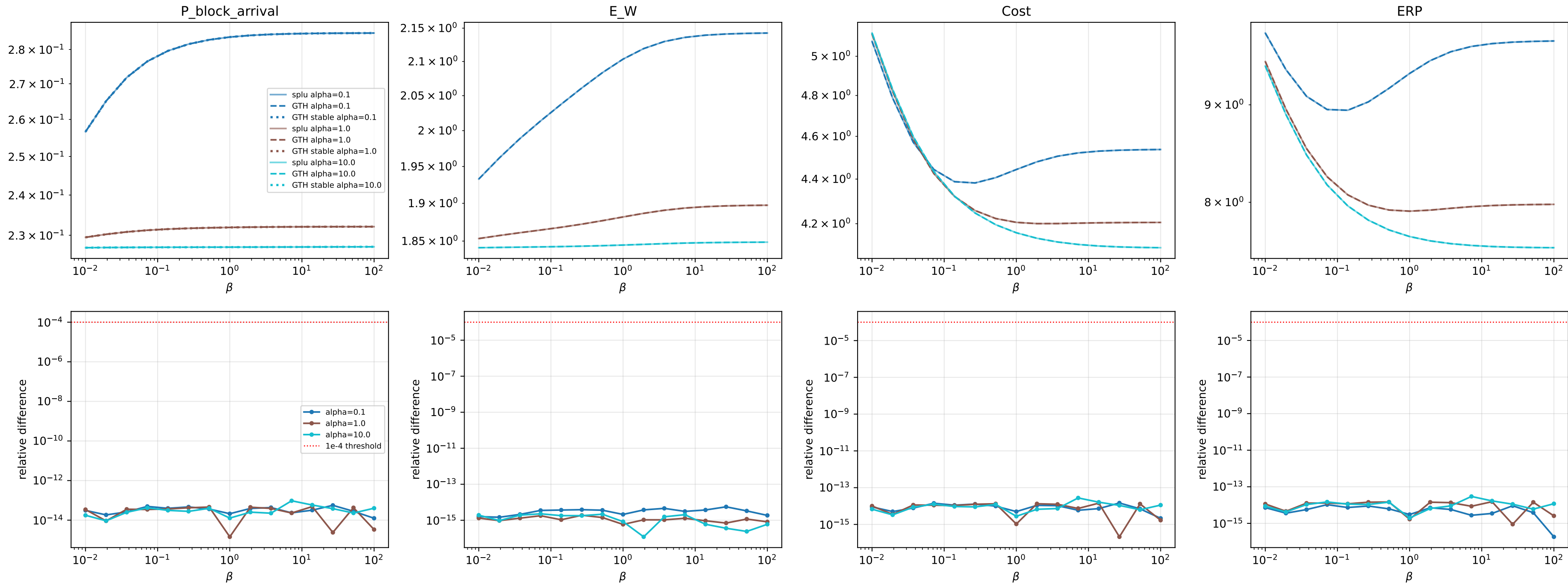
experiment_2_strong: splu (old, solid) vs GTH (new, dashed); bottom row = relative difference
