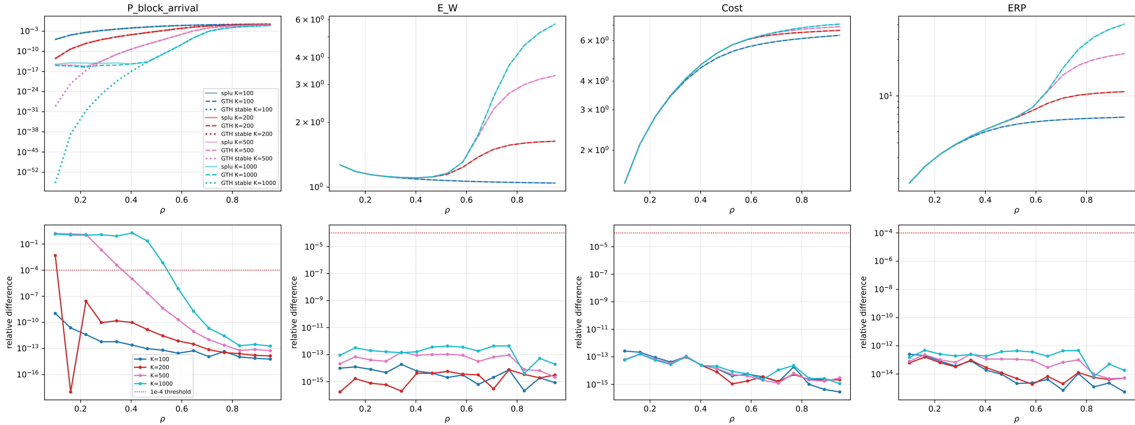
experiment_4_medium: splu (old, solid) vs GTH (new, dashed); bottom row = relative difference
