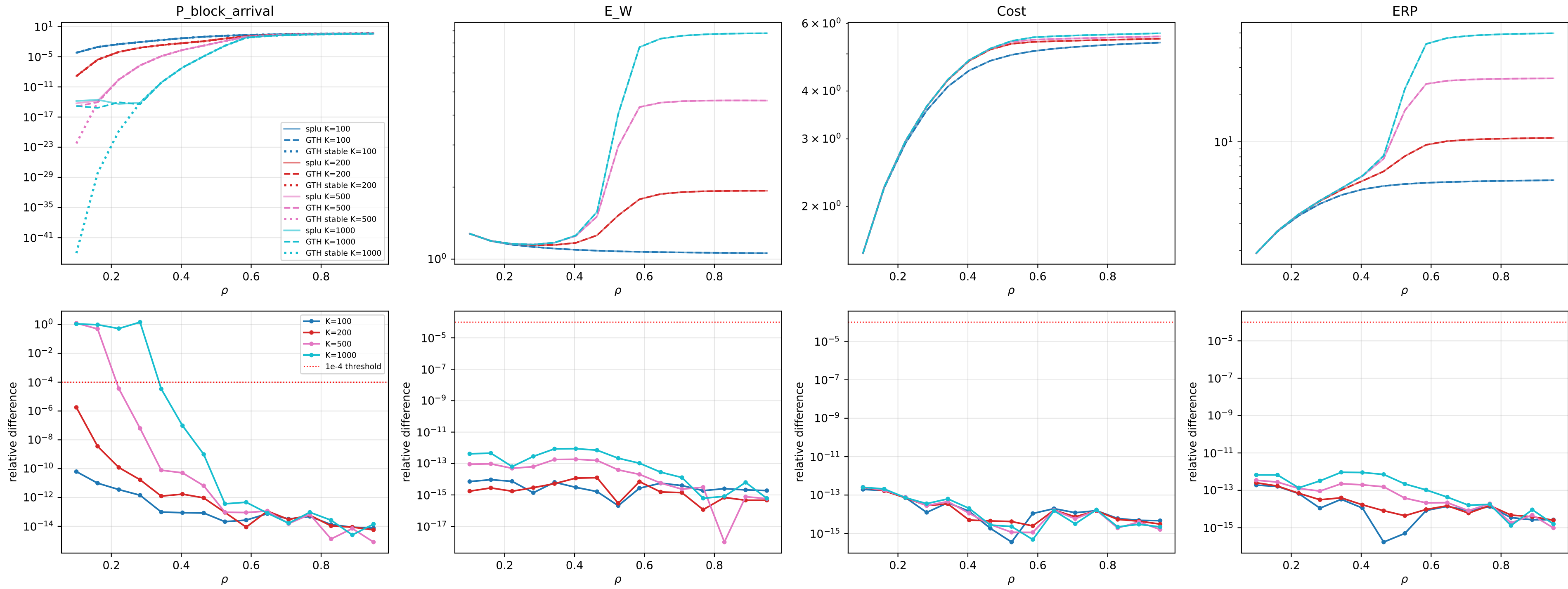
experiment_4_strong: splu (old, solid) vs GTH (new, dashed); bottom row = relative difference
