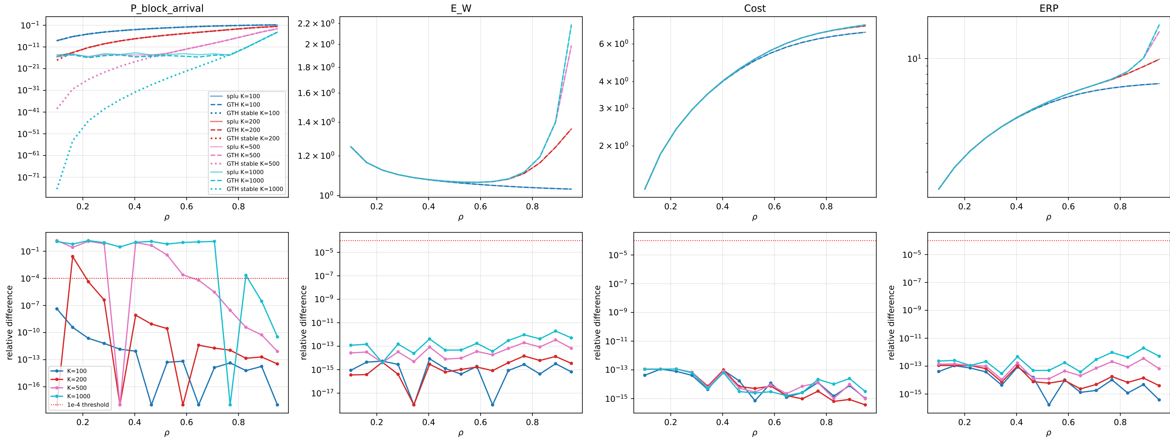
experiment_4_weak: splu (old, solid) vs GTH (new, dashed); bottom row = relative difference
