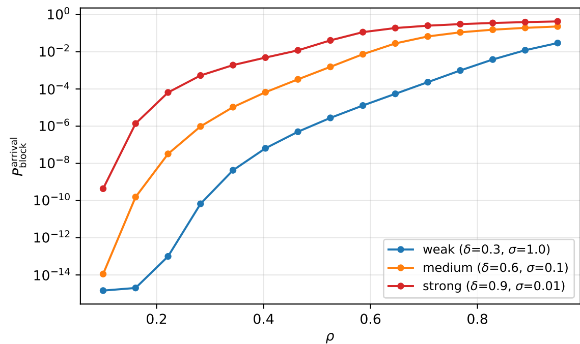
Experiment 1-P: Predictive Response to Traffic Intensity \rho (c=20, K=200, b=5, 1/alpha=10s, 1/beta=200s, n_target=10, gamma=1.0)
