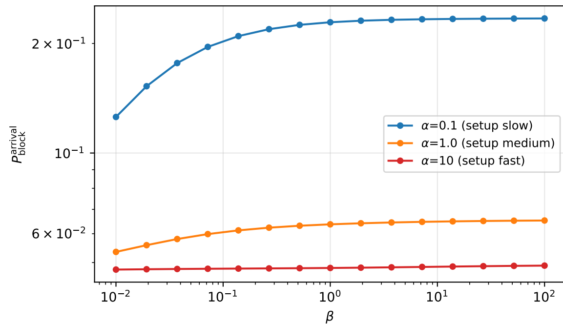
Experiment 2-P: Predictive Response to Delayoff Rate \beta (medium burst) ( c=20 , K=200 , b=5 , \rho=0.7 , n_{\text{target}}=10 , \gamma=5.0 )
