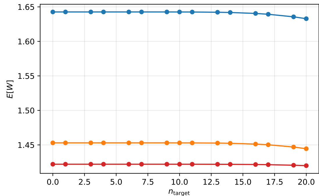
Experiment 5: Sensitivity to n_{\text{target}} (medium burst, \gamma=5.0 ) ( c=20 , K=200 , b=5 , \rho=0.7 )
