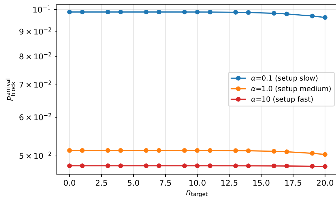
Experiment 5: Sensitivity to n_{\text{target}} (medium burst, \gamma=5.0 ) ( c=20 , K=200 , b=5 , \rho=0.7 )
