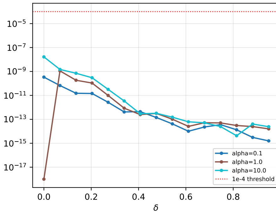
relative difference
