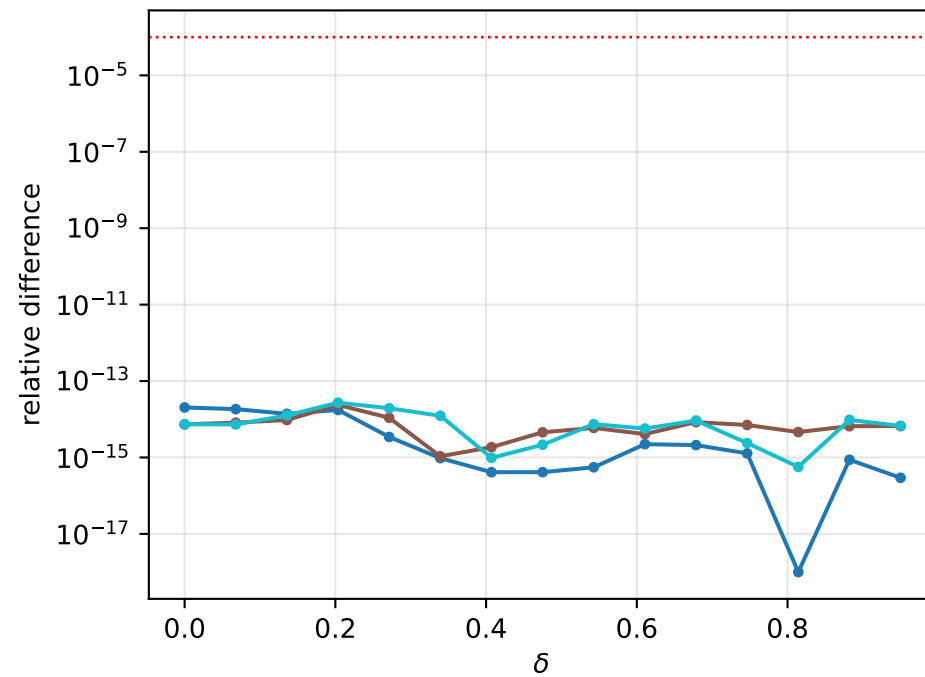
relative difference
