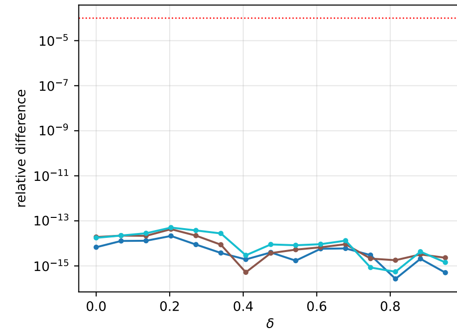
relative difference
