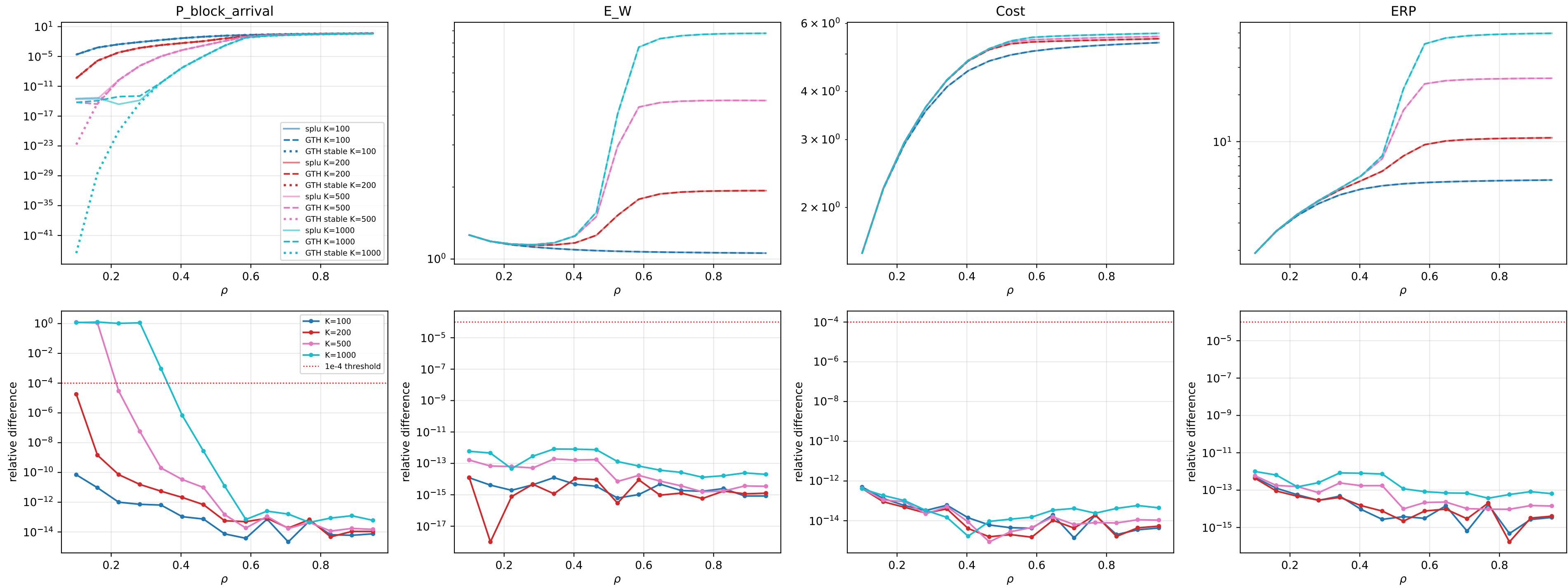
experiment_4P_strong_nt10_g1.0: splu (old, solid) vs GTH (new, dashed); bottom row = relative difference
