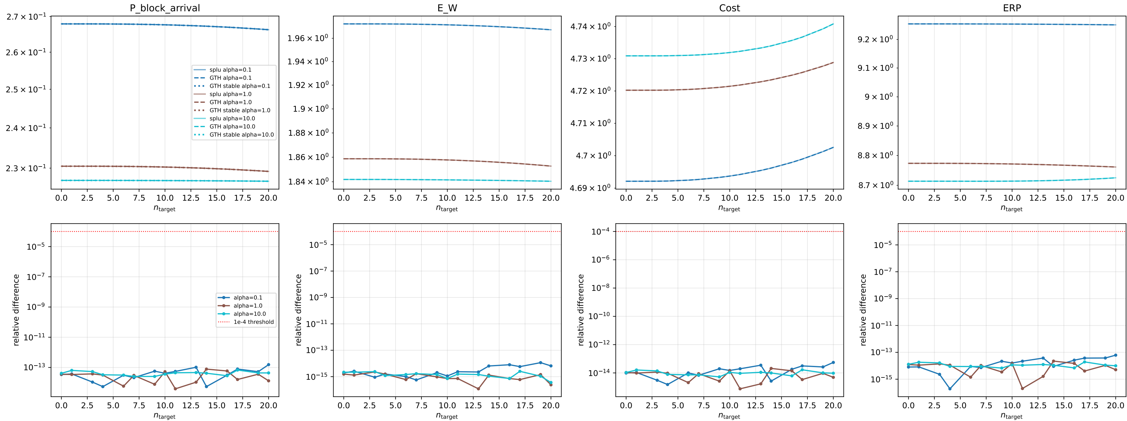
experiment_5_strong_g5.0: splu (old, solid) vs GTH (new, dashed); bottom row = relative difference
