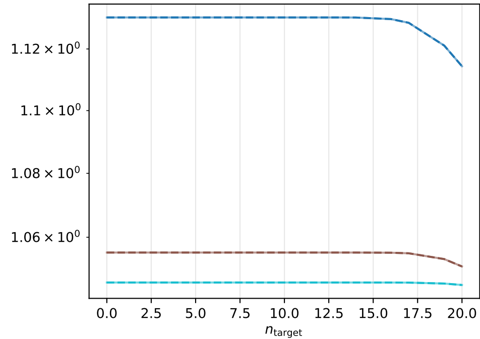
E_W
