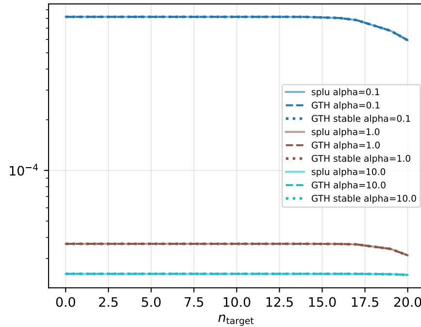
P_block_arrival
