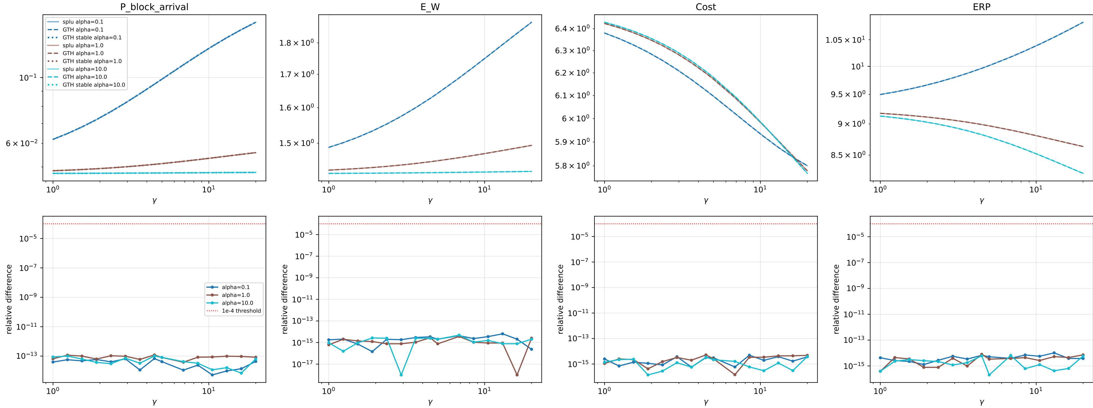
experiment_6_medium_nt10: splu (old, solid) vs GTH(new, dashed); bottom row = relative difference
