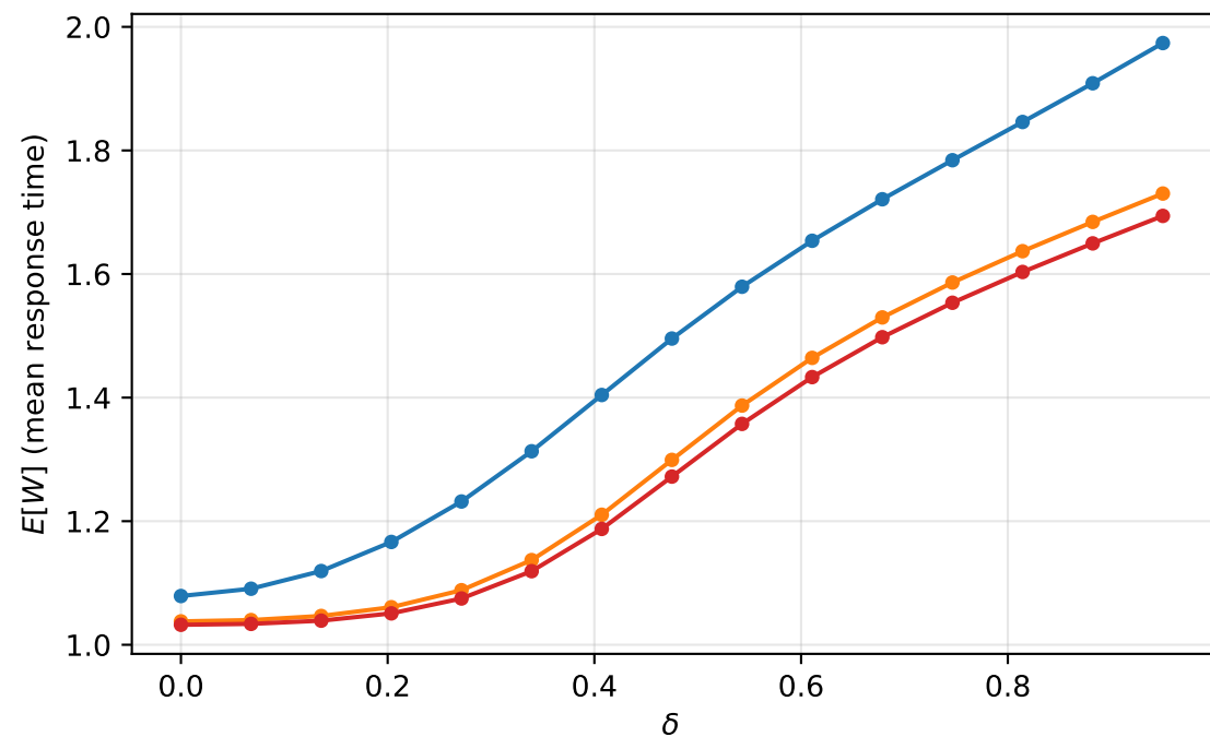
Experiment 3-P-A: Predictive Response to Burst Amplitude \delta ( \sigma=0.1 fixed) ( c=20 , K=200 , b=5 , \rho=0.7 , n_{\text{target}}=10 , \gamma=5.0 )
