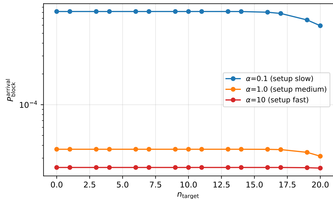
Experiment 5: Sensitivity to n_{\text{target}} (weak burst, \gamma=5.0 ) ( c=20 , K=200 , b=5 , \rho=0.7 )
