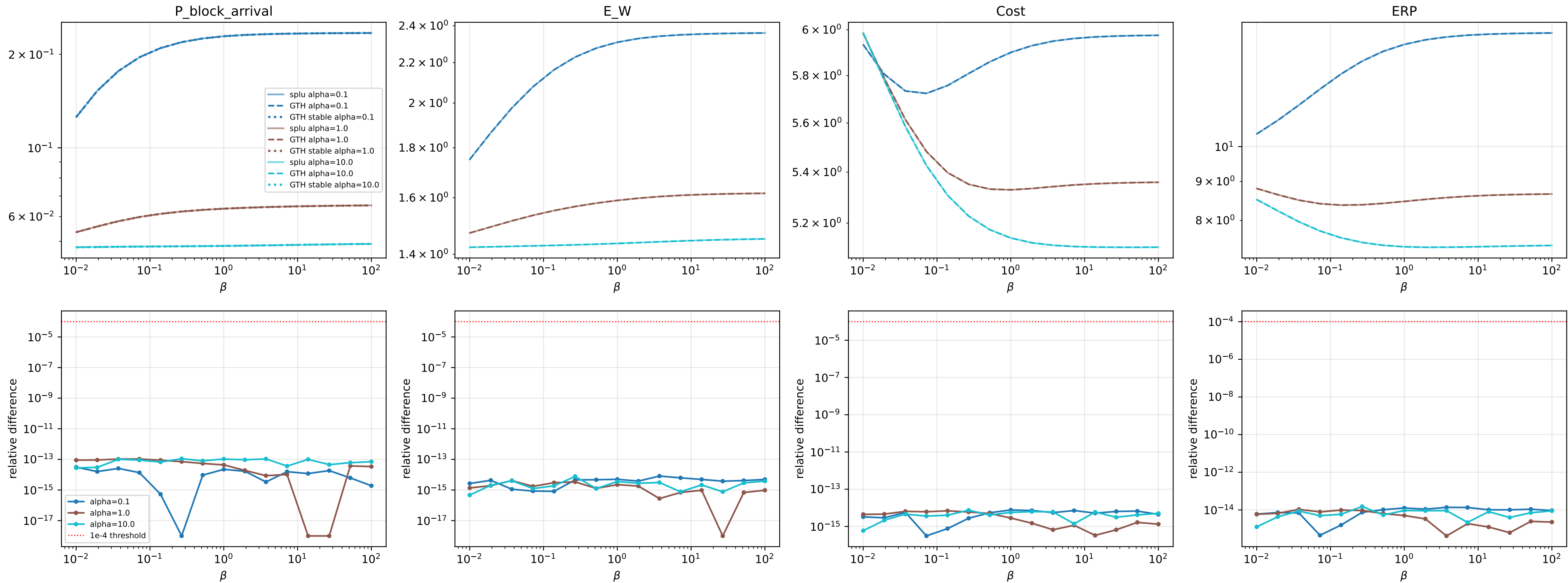
experiment_2P_medium_nt10_g5.0: splu (old, solid) vs GTH (new, dashed); bottom row = relative difference
