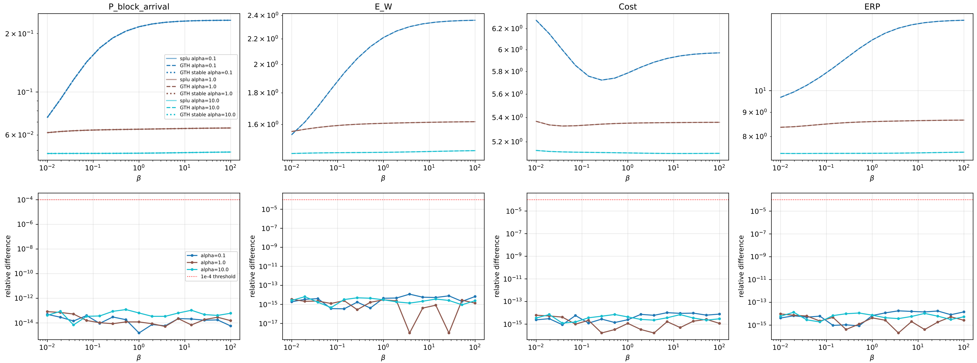
experiment_2P_medium_nt10_gmap: splu (old, solid) vs GTH (new, dashed); bottom row = relative difference
