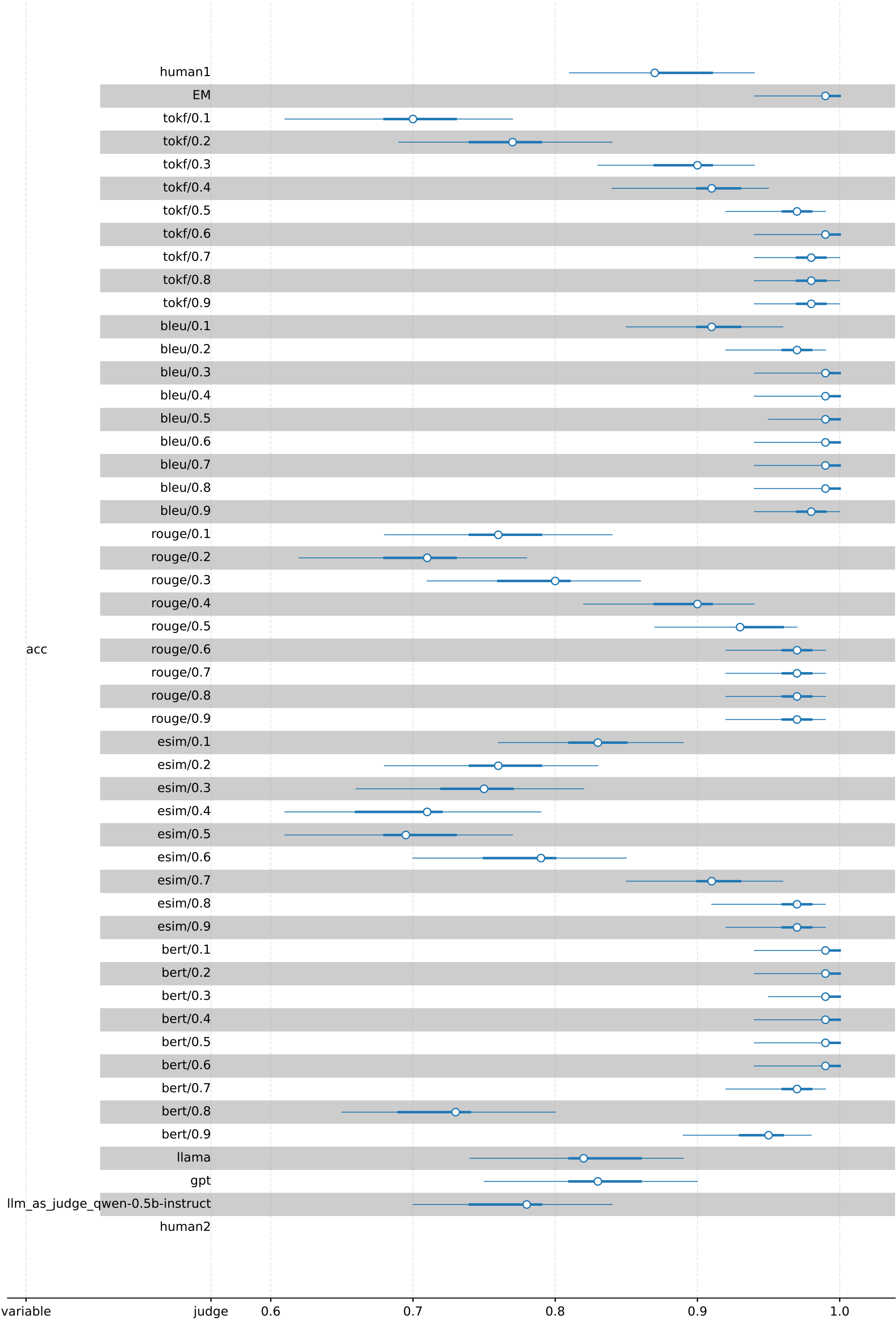
dataset=ambig_qa_single_answer generator=llama-8b-instruct | Predictive Accuracy
