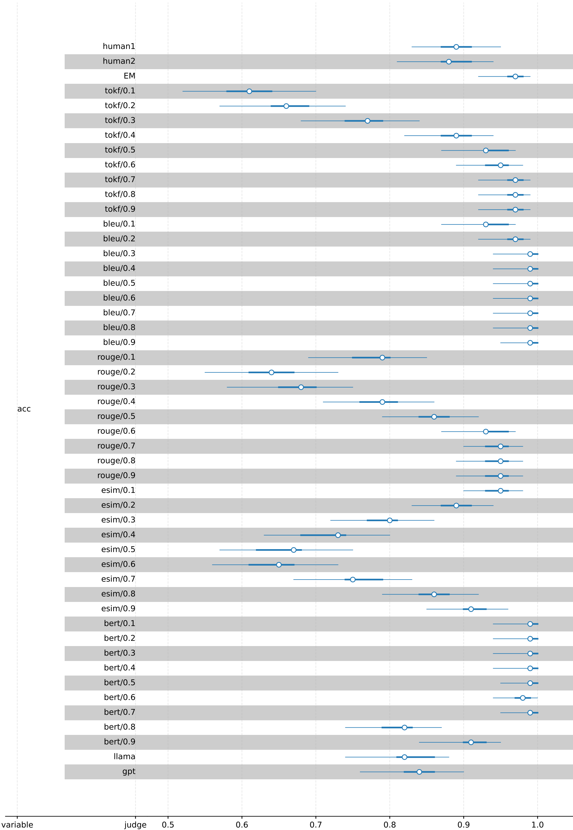
dataset=trivia_qa generator=llama-8b-instruct | Predictive Accuracy
