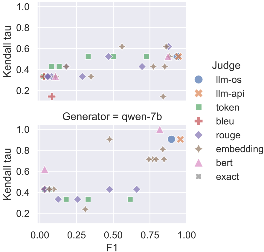
Generator = llama-8b
