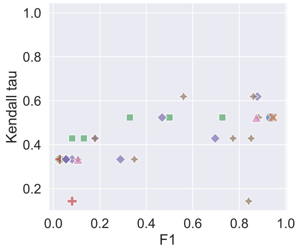
Generator = llama-8b
