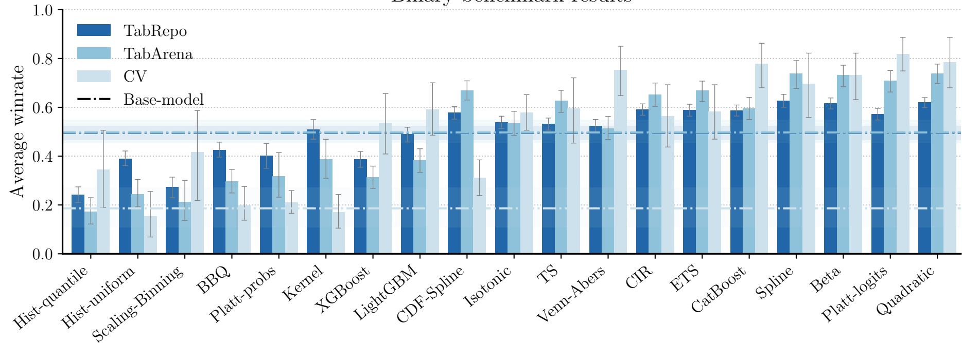
Binary benchmark results
