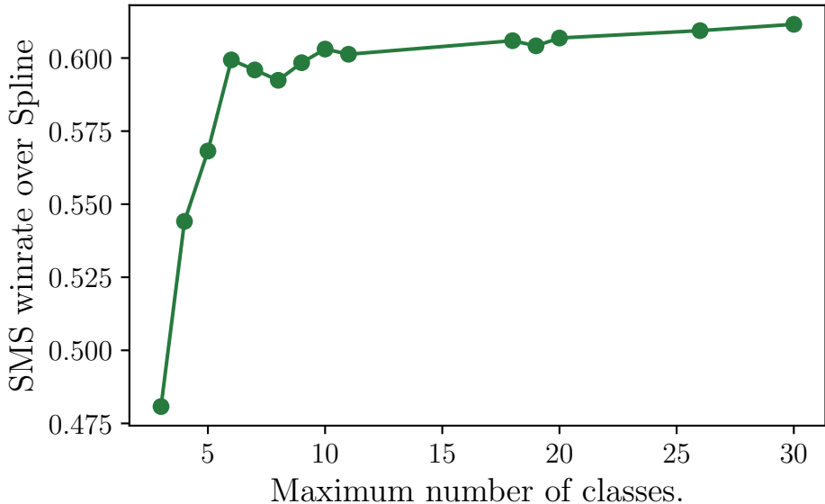
SMS vs Spline winrate, TabRepo-multiclass
