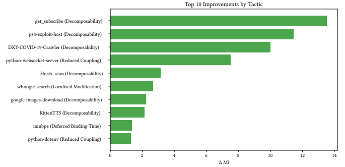
Figure 2: Top 10 MI improvements by applied tactic.
