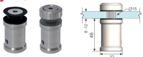
CONECTOR 32 X 46 MM.
