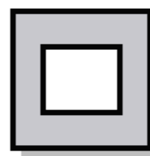
MODAL
