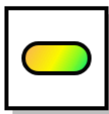
BUTTON
