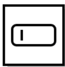
INPUT FIELD
