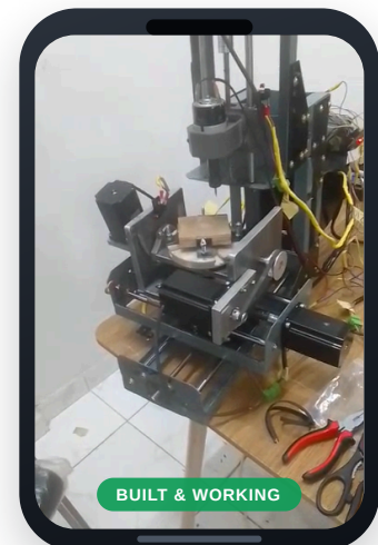
Hardware · real 5-axis rig
