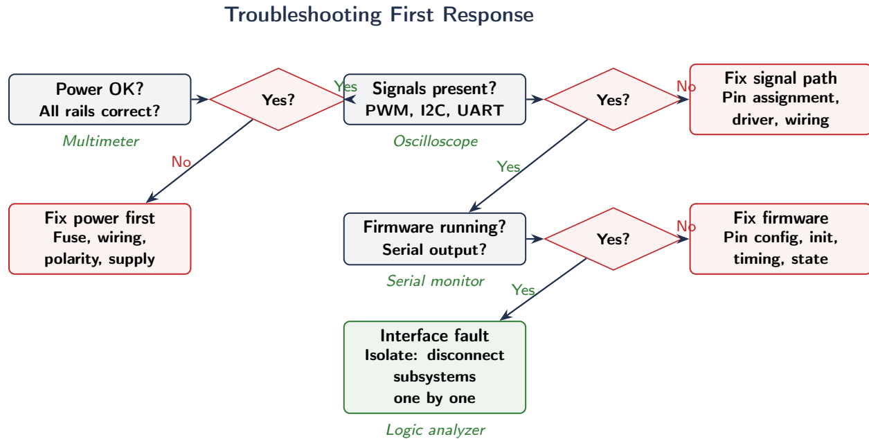
Figure 2: Troubleshooting first response. Follow left to right, top to bottom. Fix power first (most common cause), then check signals, then firmware. If all three check out, the fault is at an interface; isolate by disconnecting subsystems one at a time. See MRD Chapter 20 for the full five-step debugging protocol.
