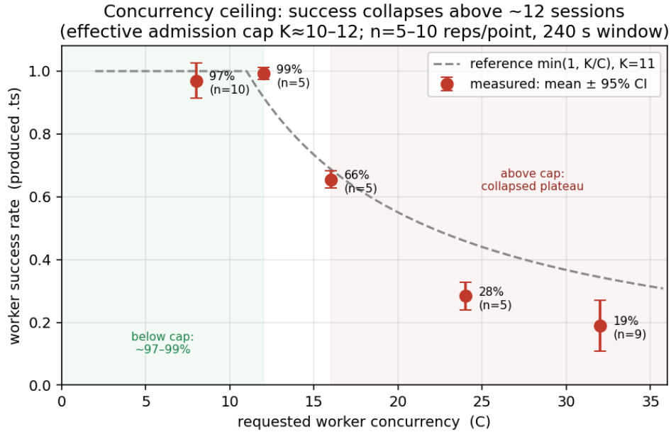
Figure 4: Replicated concurrency sweep on the full-scale (364-module) durable run, Cursor backend ( n=5-10 per point, uniform 240 s window, mean \pm 95% CI). Worker success holds at ~97–99% below ~12 simultaneous sessions and collapses monotonically above it — an effective admission cap of K \approx 10-12 imposed by the serving API, which durable state + retry then absorbs.
