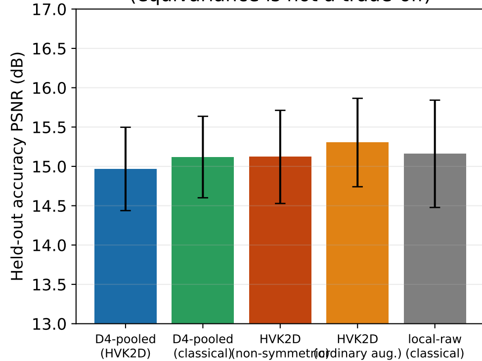
Reconstruction accuracy (equivariance is not a trade-off)
