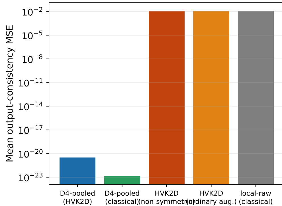
Output consistency across all 8 D4 transforms
