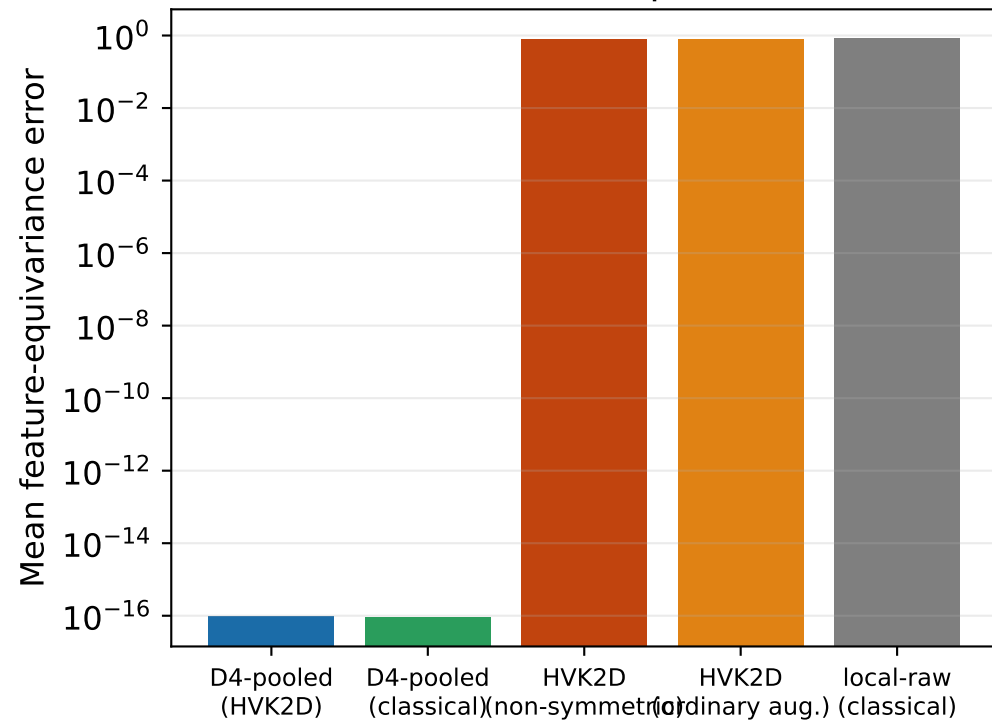
Feature equivariance (lower = more equivariant)
