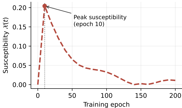
Finite-size training diagnostic
