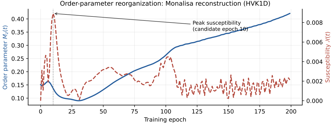
Fig. 7. Order-parameter reorganization for the actual Monalisa reconstruction run (HVK1D, the same shared-baseline checkpoint used throughout this paper), not the synthetic restricted diagnostic. Curves and axes follow Figure 6. The candidate reorganization epoch is t_c = 10 with \lambda_{\max} = 0.0089 , an order of magnitude smaller than in the synthetic diagnostic and selected by the same median-plus-two-standard-deviation rule; M_z(t) continues to climb as training proceeds toward the final 40.70 dB reconstruction.
