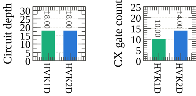
Fig. 10. IBM Cloud circuit-resource summary for the HVK1D and HVK2D hardware probes.
