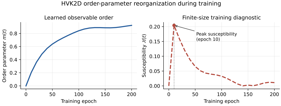
Fig. 6. Order-parameter reorganization for the HVK2D entangling baseline on the restricted pair-correlation diagnostic. The solid blue curve is M_z(t) ; the dashed red curve is \mathcal{X}(t) = |M_z(t) - M_z(t - \Delta t)| . The dotted line and arrow mark the candidate reorganization epoch t_c = 10 , where \mathcal{X}_{\max} = 0.204 . This is the point of fastest observed change under Eqs. (2)–(3), not a thermodynamic critical point.
